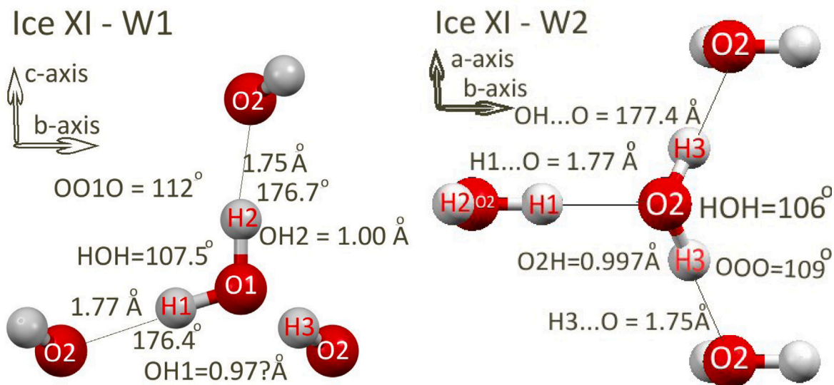
Fig. 11. Graphical summary of plausible Ice XI structure, left: showing W1, viewed down a -axis; right: showing W2, viewed down c -axis.
